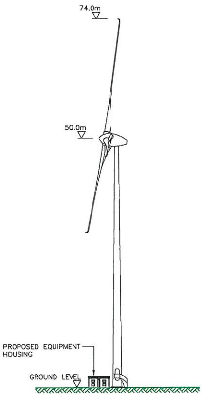
SIDE ELEVATION (1:500)
